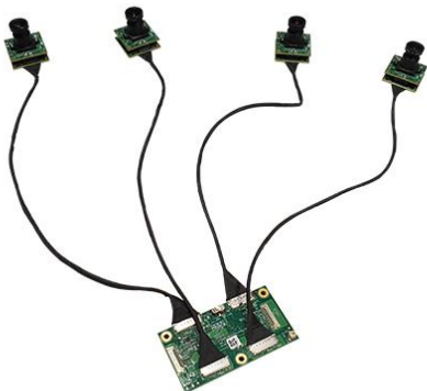
Fig:1 SurveilsQUAD Synchronized Multi-camera Systems
