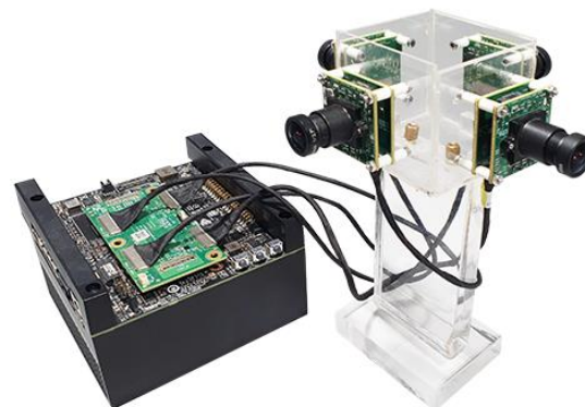
Fig:2 – SurveilsQUAD connected to NVIDIA Jetson Xavier
